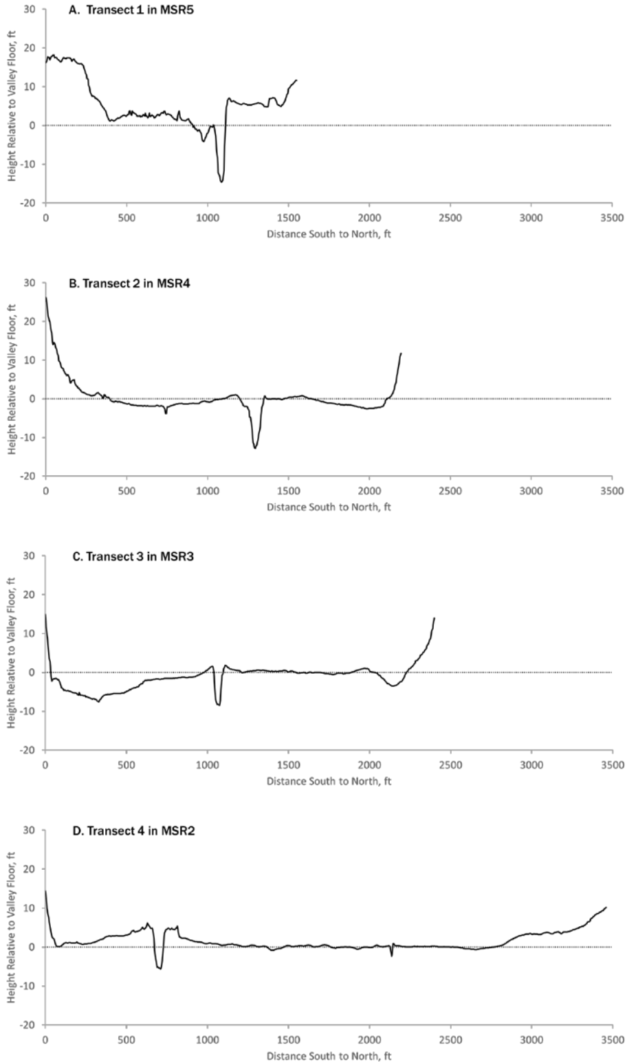
Figure 3-4. Longitudinal changes in cross sectional valley form. Refer to Figure 3-1 for the location of valley transects.
