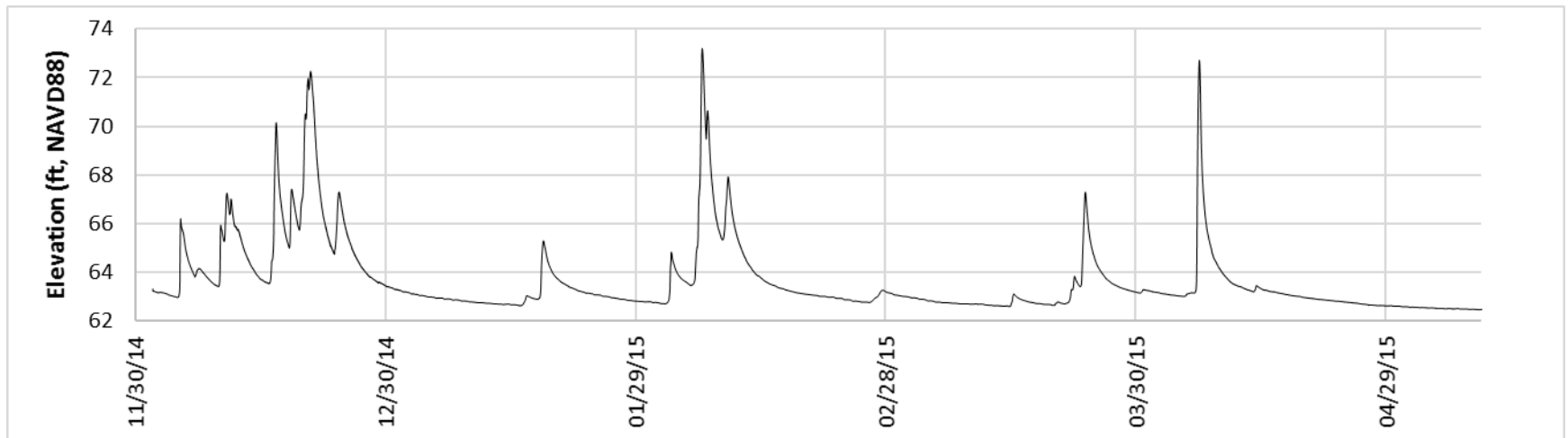
Figure 4-16. Continuous water surface elevation measurements for SFR2 (Dec. 2, 2014–May 11, 2015).
