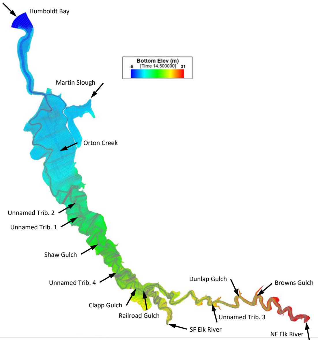
Figure 5-2. ER-HST model grid and boundary conditions.
